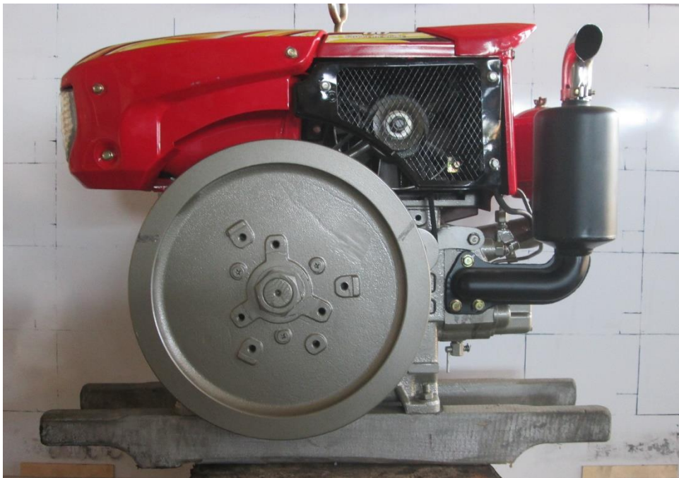
Figure 1. KATO KD80N PH Diesel Engine
