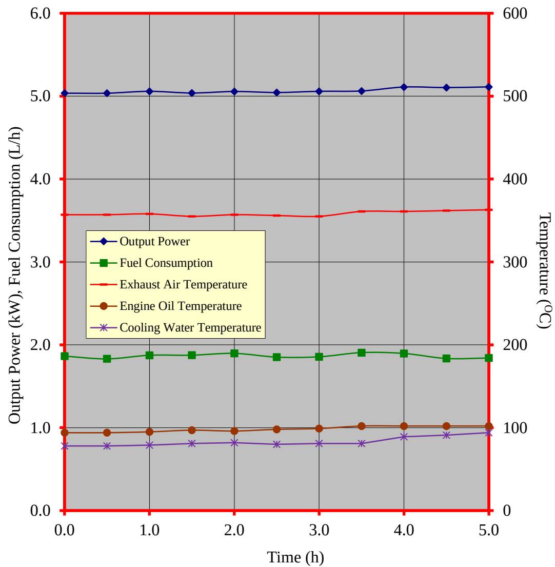
Figure 4. Performance characteristic curves during the continuous running test of the KATO KD80N PH diesel engine
