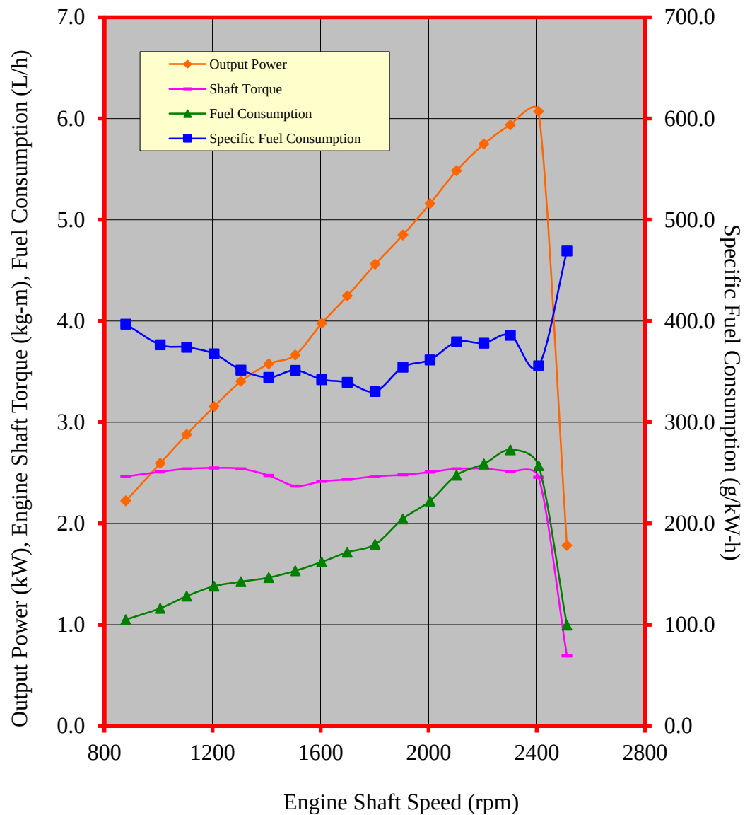
Figure 3. Performance characteristic curves of the KATO KD80N PH diesel engine
